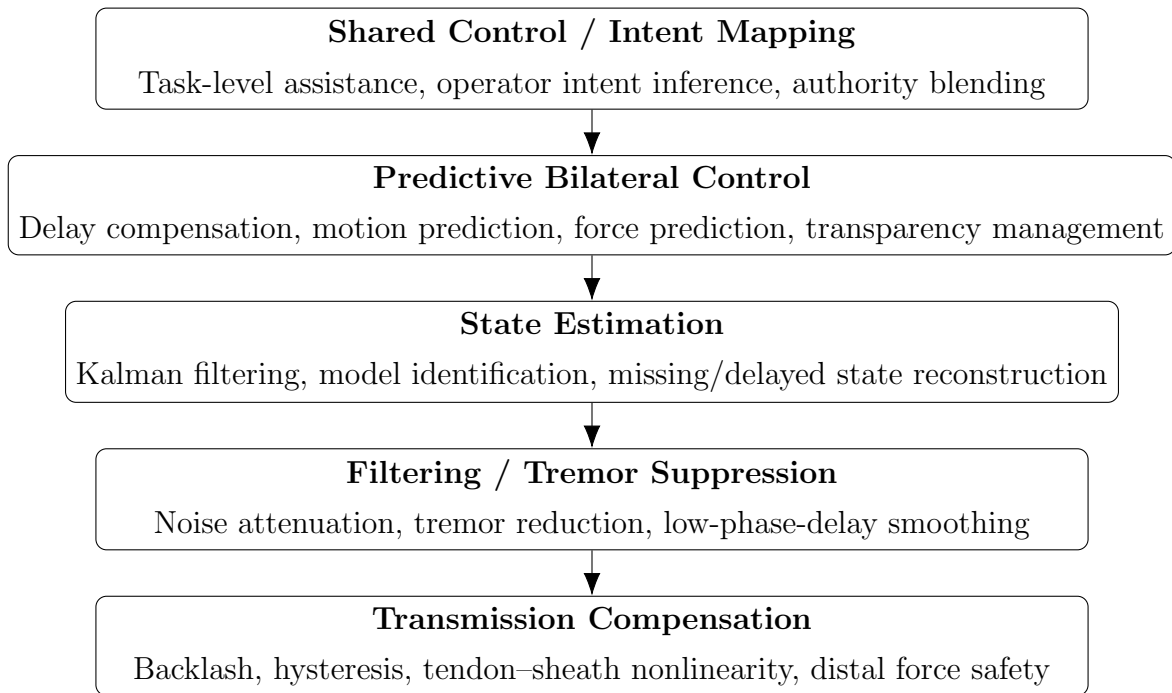
Figure 4: Linked control layers relevant to teleoperation in macro-micro surgical robotics. The literature reviewed in this subsection can be interpreted across these interacting layers, from low-level transmission effects to high-level shared control.
